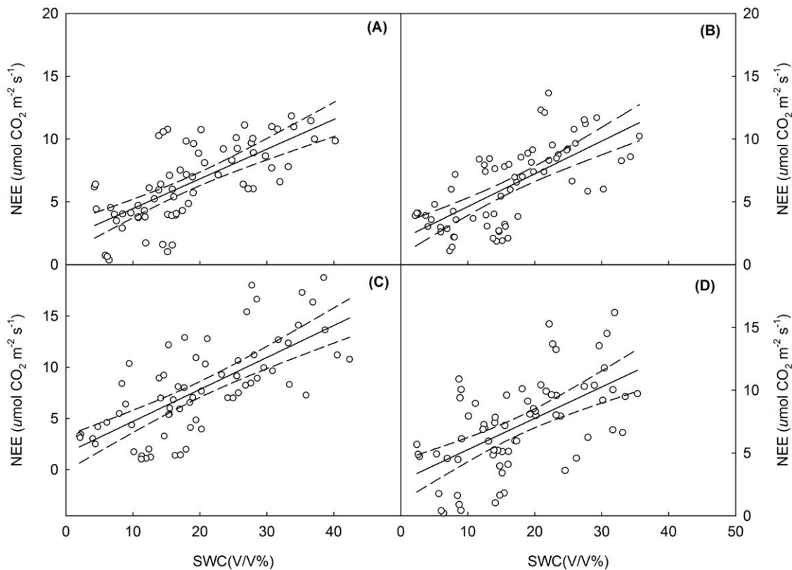
Figure 4. Temporal dependence of net ecosystem \text{CO}_2 exchange (NEE) on soil water content (SWC) across the four growing seasons. Regression lines (solid) and 95% confidence level (dotted lines) are shown. All the linear regressions are statistically significant ( P < 0.05 ). Regression equations and significance levels are provided in Table 4. (A), control; (B), warming; (C), N addition; (D), combined warming and N addition. doi:10.1371/journal.pone.0045205.g004
